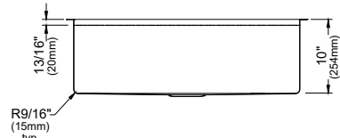
MODEL: WS-37-D1-PK1 Stainless Steel Undermount Single Bowl Workstation Sink
