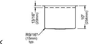
MODEL: WS-31-D1-PK1 Stainless Steel Undermount Single Bowl Workstation Bar Sink
